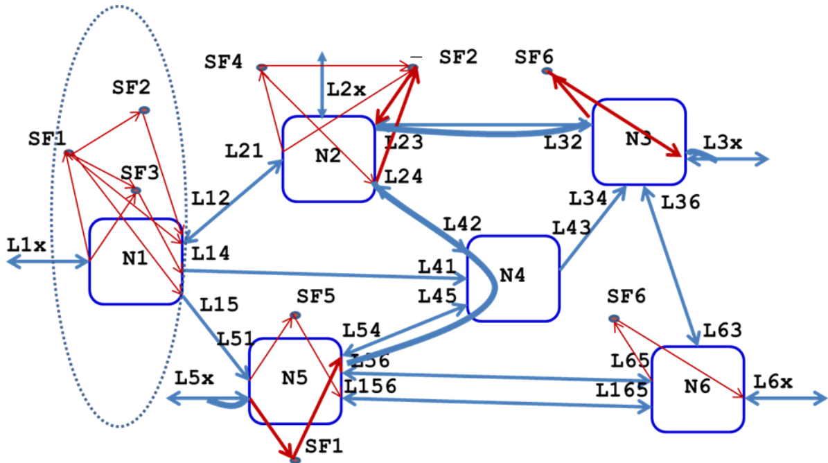
Figure 5: SFC recovery: SFC SF1-SF2-SF6 is recovered after SF2 on node N1 has failed
