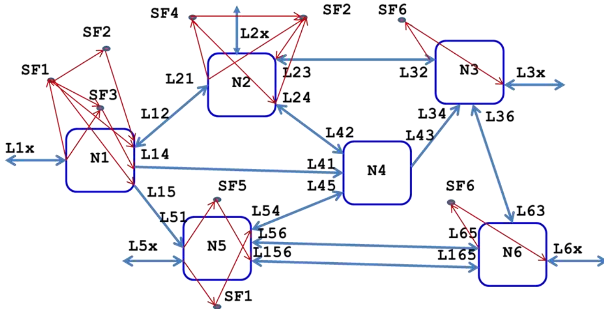
Figure 1: SF/NF aware TE topology
